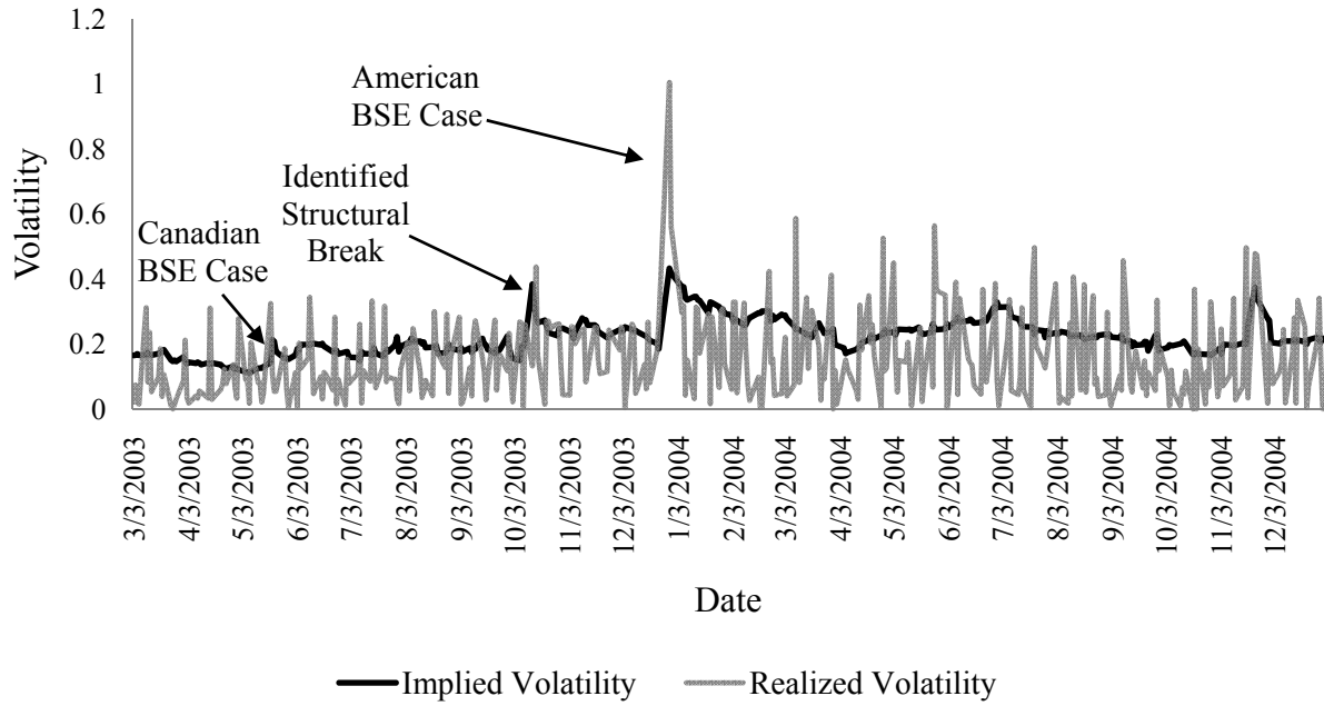
Figure 1. Live Cattle Daily Implied and Realized Volatility, 3/2003-12/2004
