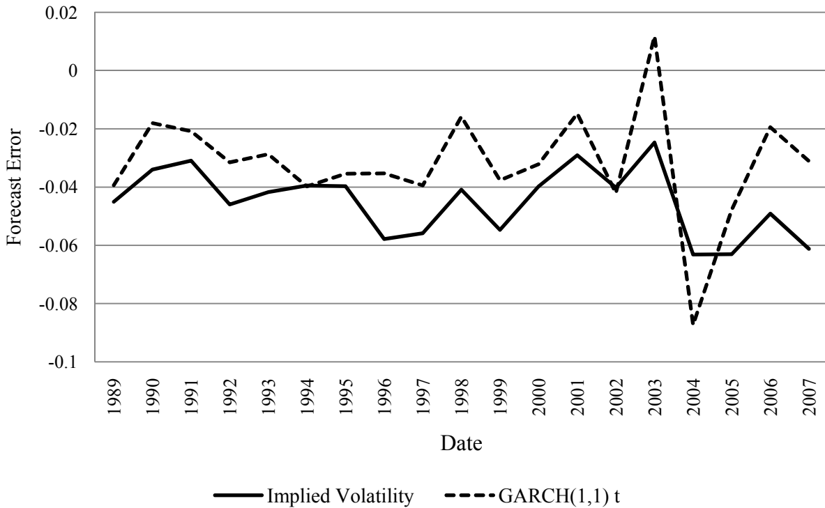
Figure 7. Live Cattle Average Annual Weekly Forecast Error, 1/1989-1/2008
