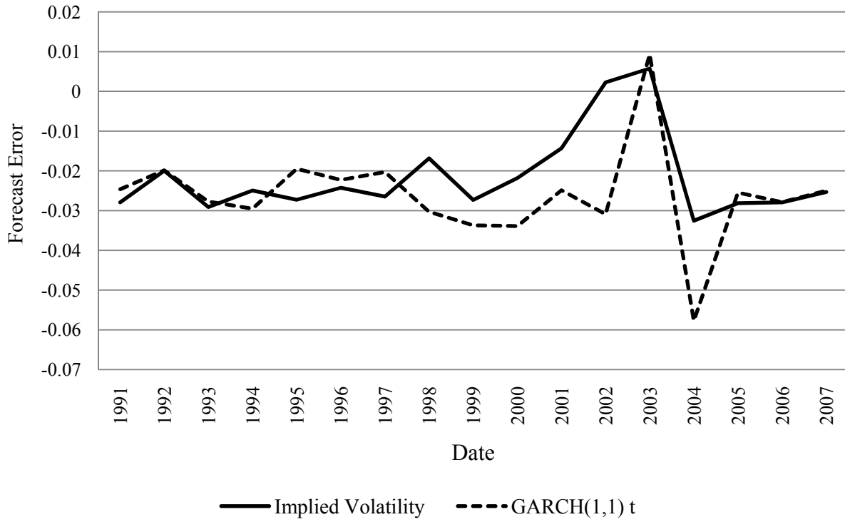
Figure 8. Feeder Cattle Average Annual Weekly Forecast Error, 3/1991-1/2008
